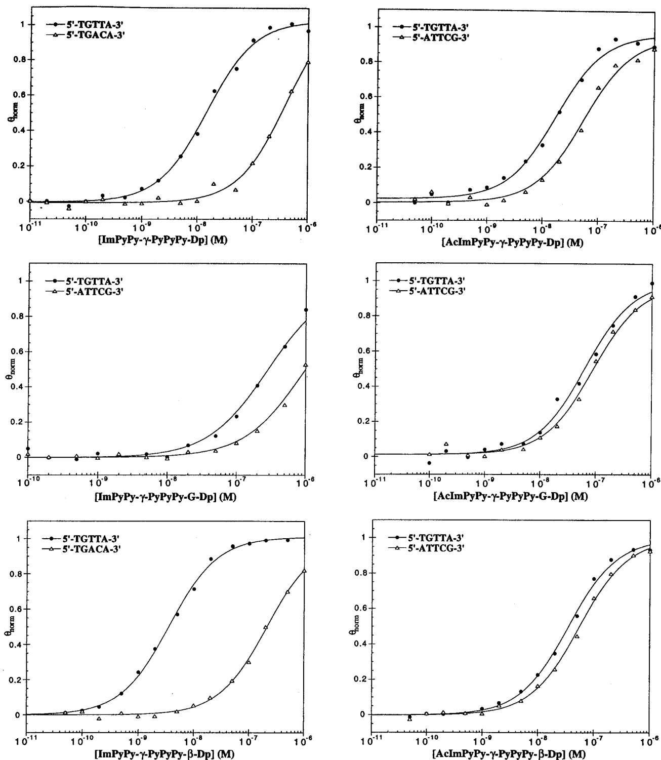
Figure 6. Data for the quantitative DNase I footprint titration experiments for the six polyamides in complex with the designated 5'-TGTTA-3' target site. The \theta_{\text{norm}} points were obtained using photostimulable storage phosphor autoradiography and processed as described in the Experimental Section. The data points for ImPyPy- \gamma -PyPyPy-Dp (1), ImPyPy- \gamma -PyPyPy-G-Dp (3), ImPyPy- \gamma -PyPyPy- \beta -Dp (5), AcImPyPy- \gamma -PyPyPy-Dp (2), AcImPyPy- \gamma -PyPyPy-G-Dp (4), and AcImPyPy- \gamma -PyPyPy- \beta -Dp (6) are indicated by filled circles for the 5'-TGTTA-3' match site, and open triangles for the 5'-TGACA-3' or 5'-ATTCG-3' single base pair mismatch sites. The solid curves are the best-fit Langmuir binding titration isotherms obtained from nonlinear least squares algorithm using eq 2.
